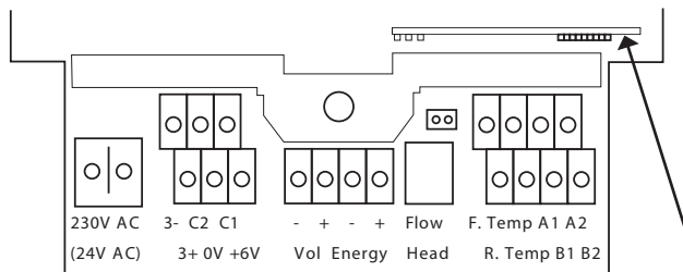
Fig 37: Communication module connection
